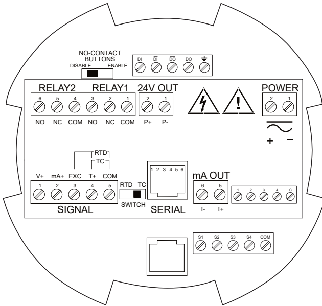
Connections on Back of PD8-765 Electronics Module (PD8-765-6X5-10 shown)
