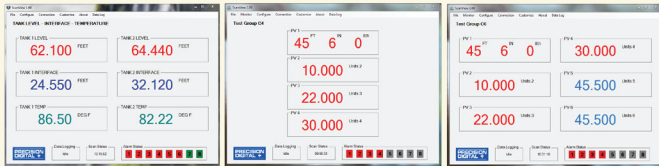
Resident on PD6080/81 Modbus Scanners
